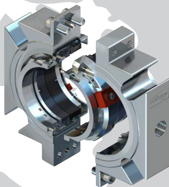
PSS4 Split Seal
