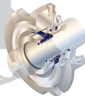
ISC2 Single Seal
